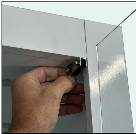
14. Attach the top hinge to display case and insert the glass door.
